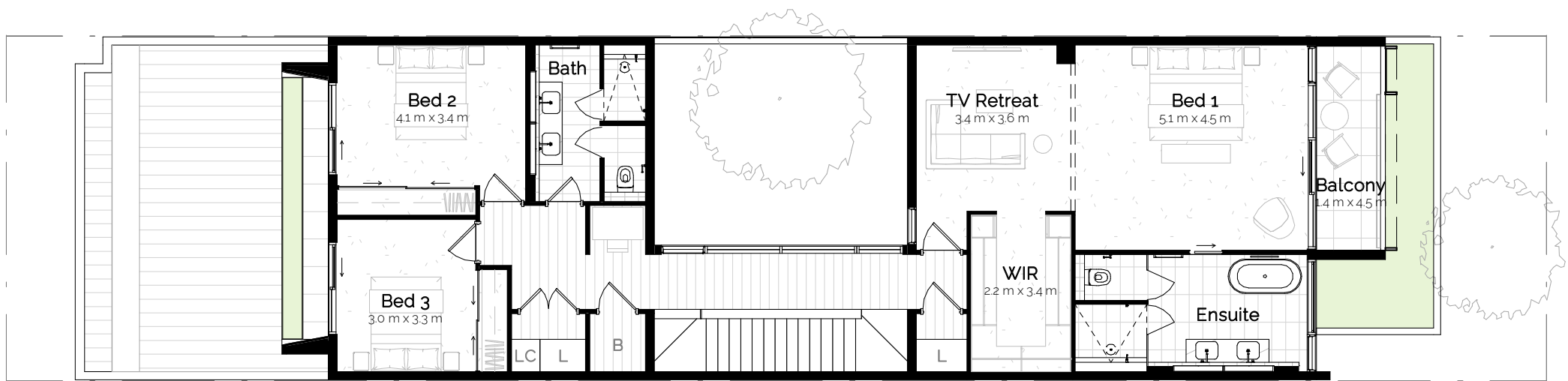
FIRST FLOOR
